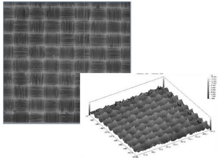
Measurement of Transparent and Soft Media e.g. Polymer Diaphragm
